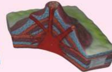
Volcano Model
